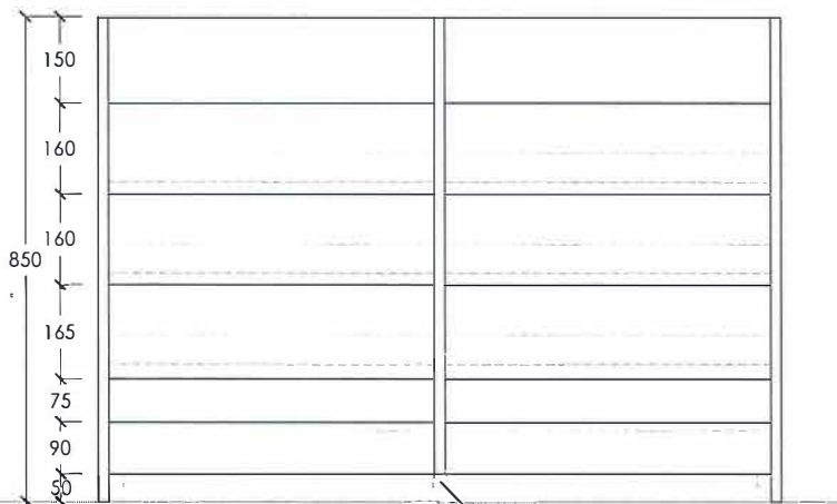
VISTA FRONTAL
