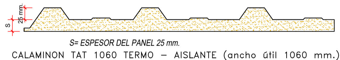
PLANCHA CALAMINON
